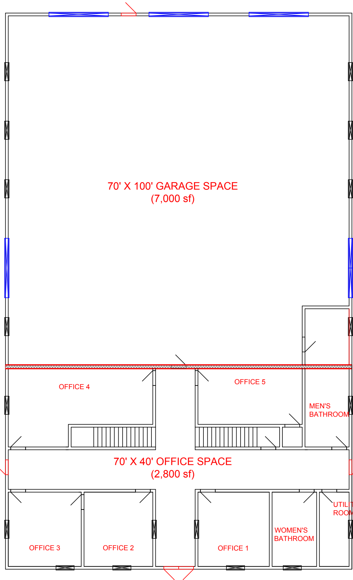
1st floor & garage
