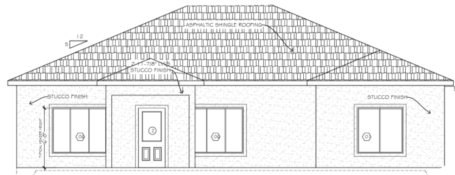
Rear Elevation
