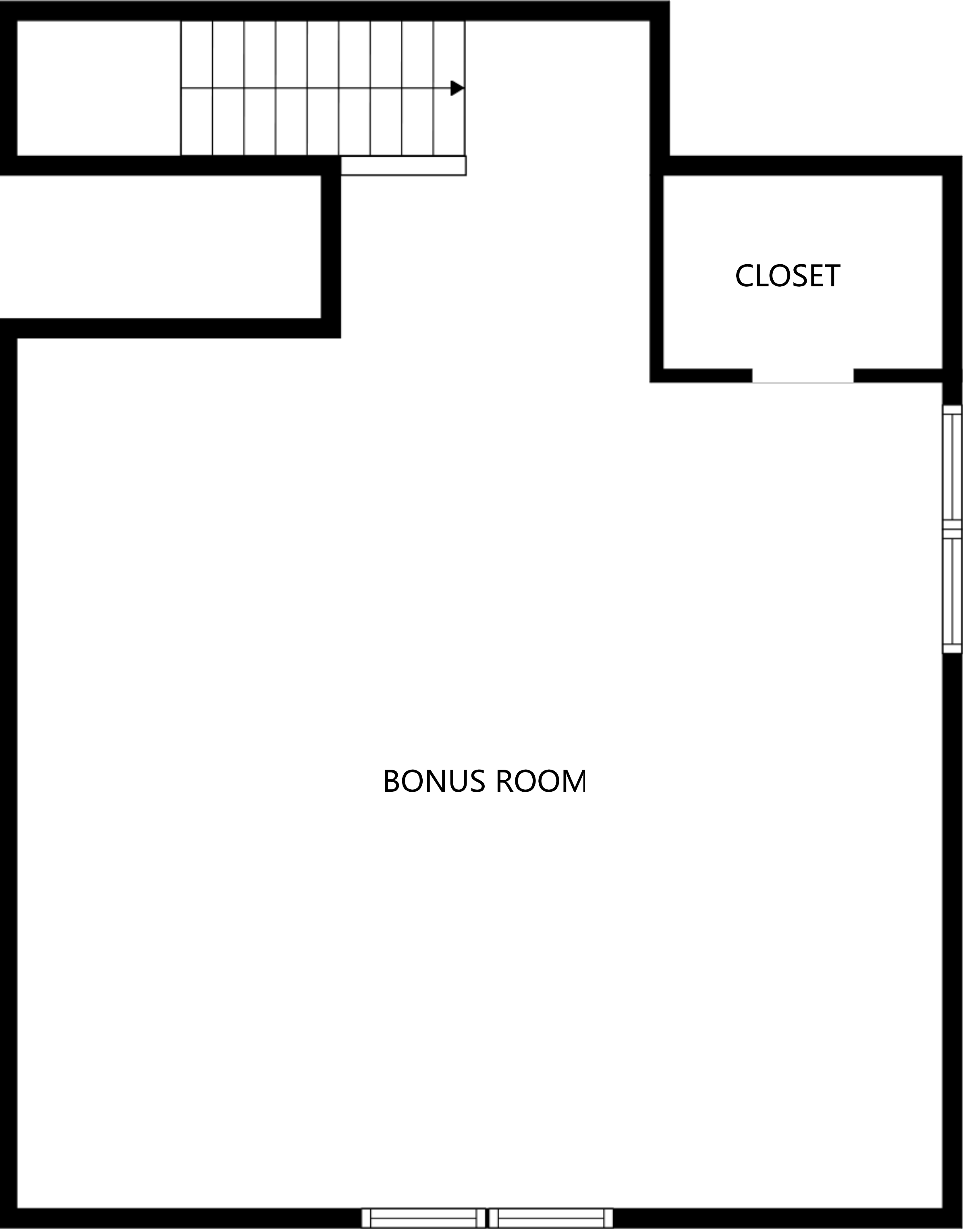
FLOOR 2 Second Floor Living Area: 723 sq ft
