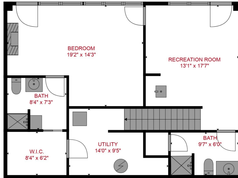
FLOOR 2
