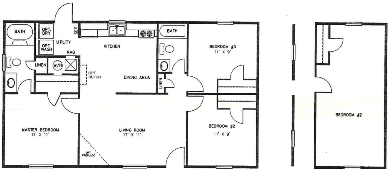
STYLE:2444 (Approx. 907 Sq. Ft.) Model #HA24403A
