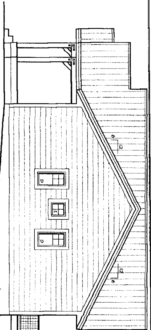
RIGHT ELEVATION 3/8" = 1'-0"
