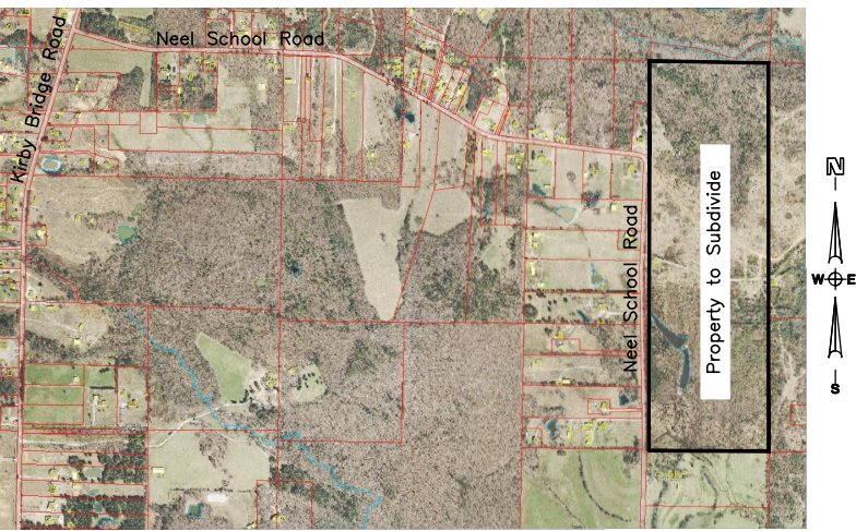
Vicinity Map (1"=1000')
